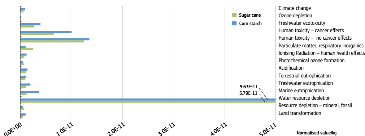
Figure 25: Normalised environmental impacts of polyhydroxyalkanoates production
