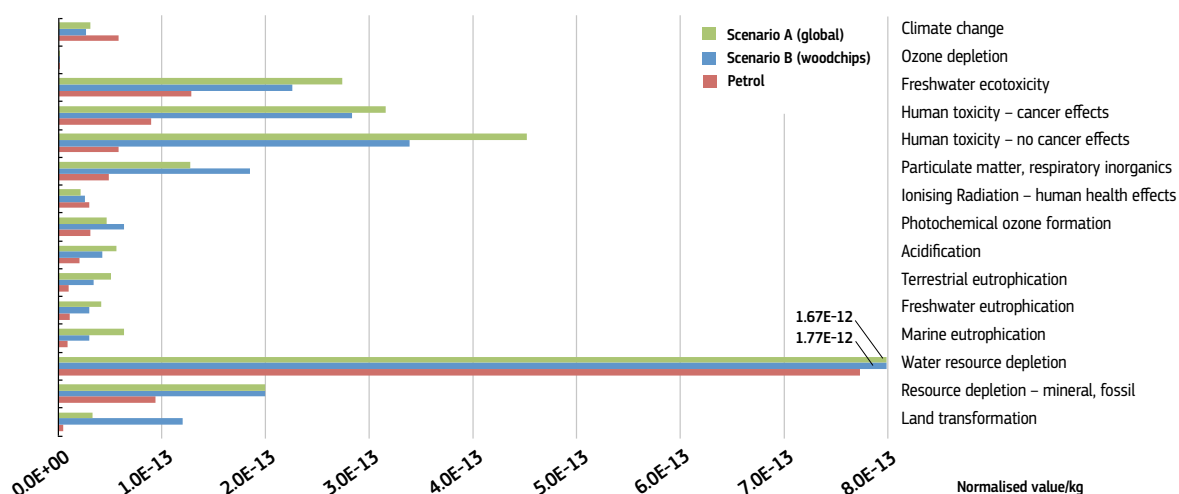
Figure 24: Normalised environmental impacts of bio-based ethanol production
